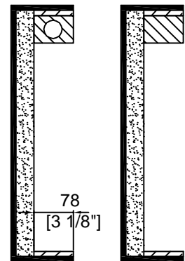
D-D VIEW E-E VIEW
